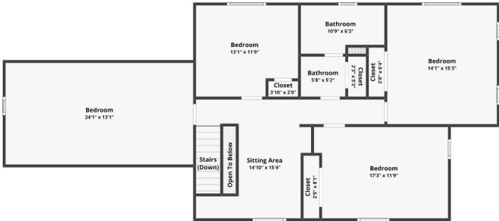
FLOOR 2 Finished area: ~1,227.54 sq. ft. Unfinished area: ~1.77 sq. ft.
